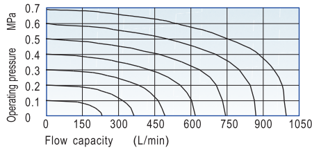
Model: 3L110-06
